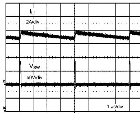
FIGURE 5. Short Circuit at 48V IN
