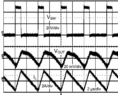
FIGURE 9. Synchronous Operation at 48V IN with JMP1 Removed
