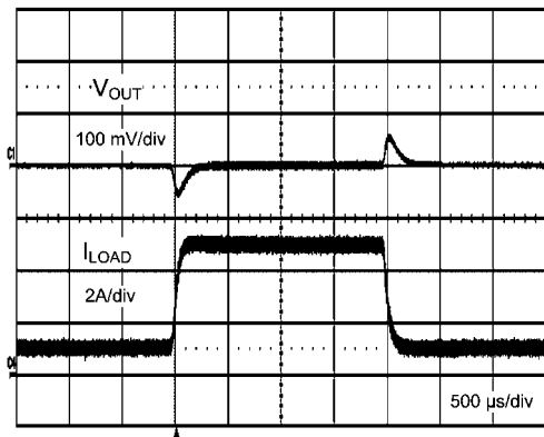
FIGURE 11. Transient Response at 48V IN
