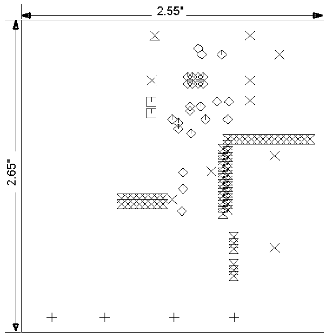
DRILLS AND DIMENSIONS (.FAB) LAYER AS VIEWED FROM TOP 880013185-002
