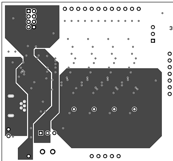
FIGURE 9. LP5521 Evaluation Board Layer 3 (Power).
