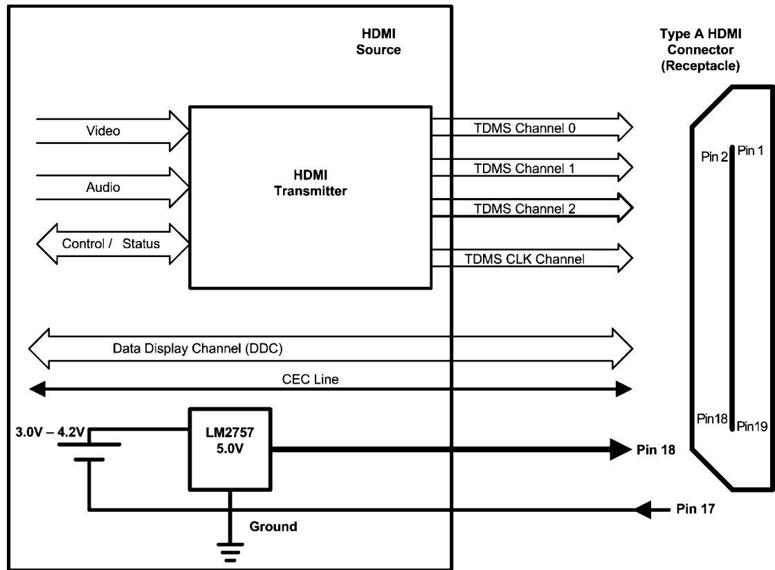
FIGURE 1. HDMI System Block Diagram
