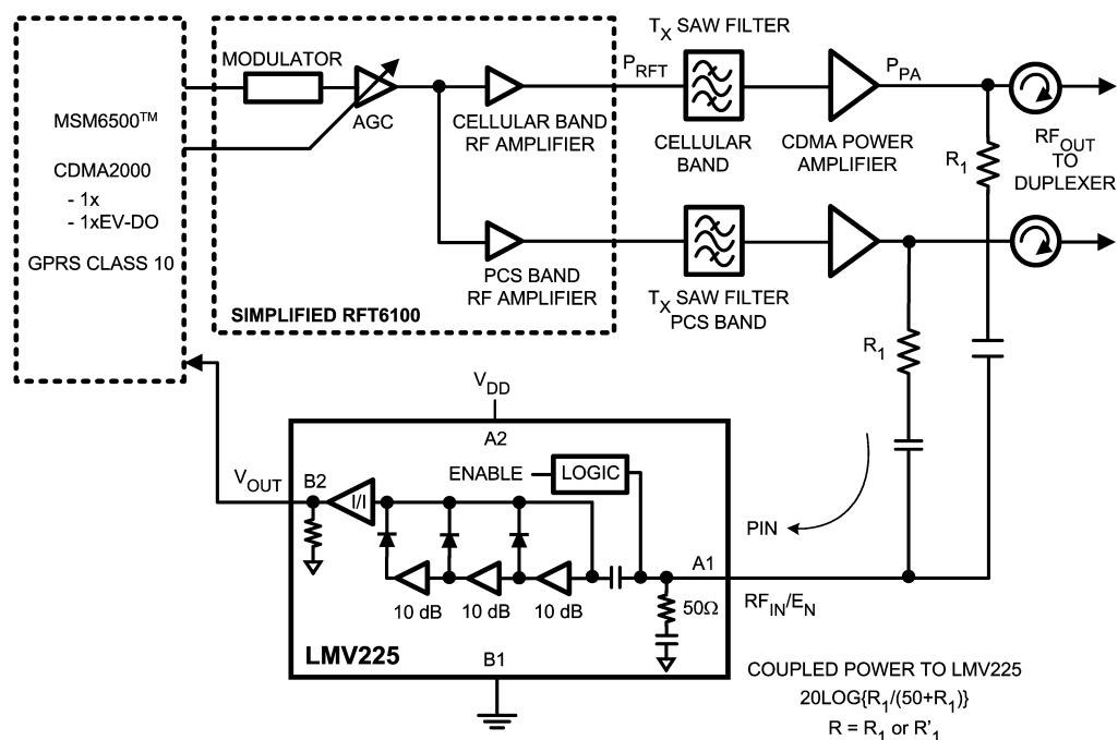
FIGURE 8. Dual-Band CDMA2000 Transmit Architecture
