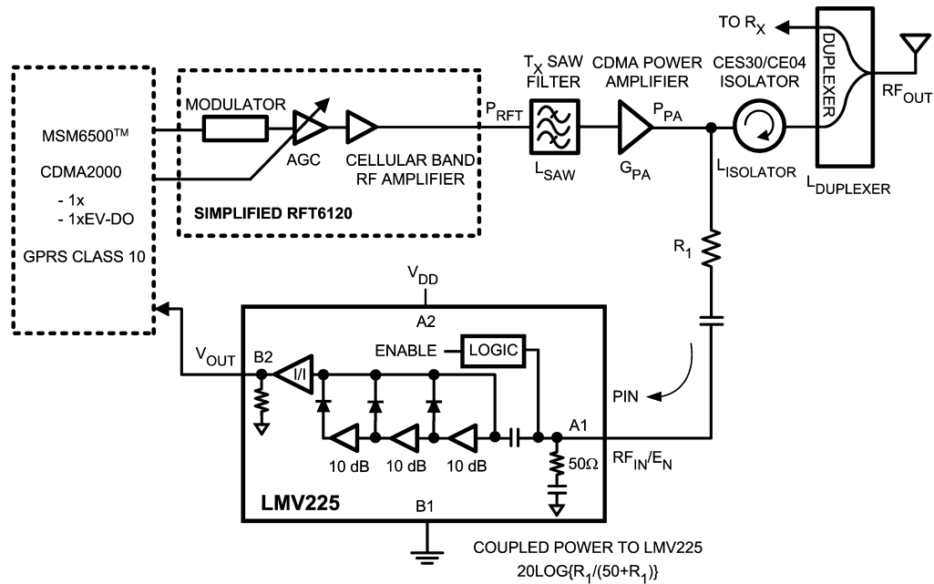
FIGURE 5. Single-Band CDMA2000 T x Architecture
