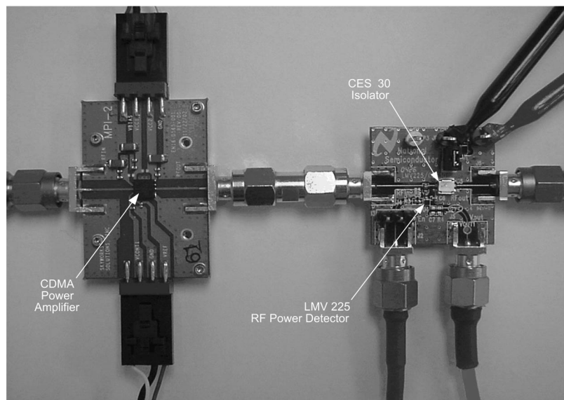
FIGURE 4. LMV225 Eval Board + CDMA PA's Module
