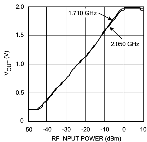
FIGURE 7. Typical Performance at DCS/PCS/W-DCMA Bands
