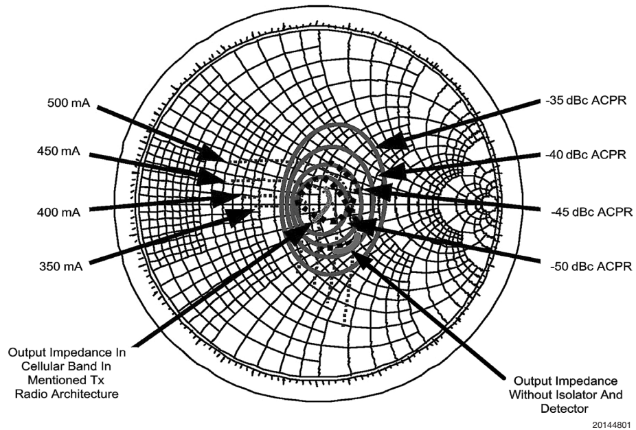
FIGURE 3. Output Impedance Smith Chart
