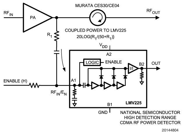
FIGURE 2. Transmit Radio Architecture
