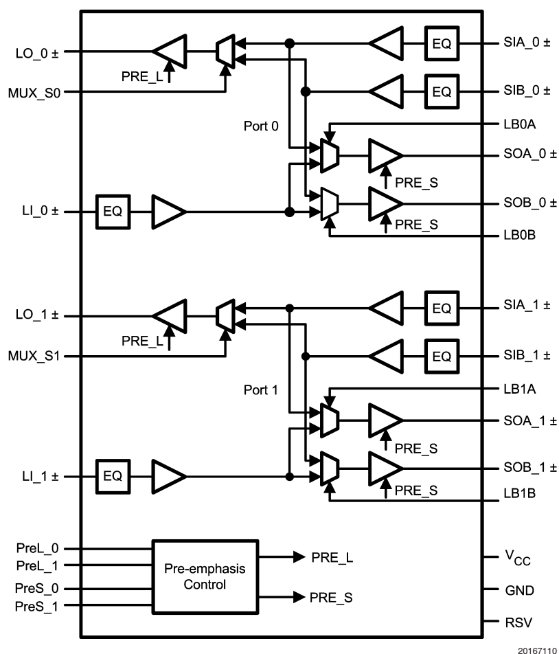
FIGURE 1. Functional Block Diagram of the DS40MB200
