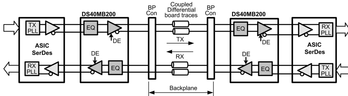
FIGURE 5. DS40MB200 as an Equalizer used with ASIC/SerDes
