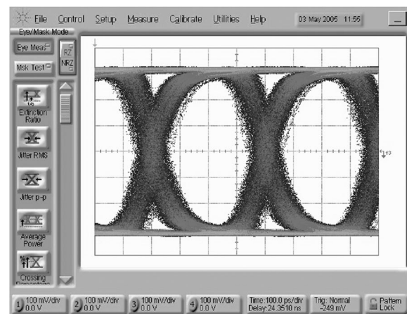
FIGURE 8. Data Eye Pattern after a 10-Meter CAT7 Cable at 2.5 Gbps
