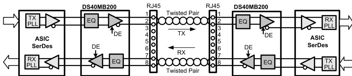
FIGURE 6. DS40MB200 as a Cable Equalizer
