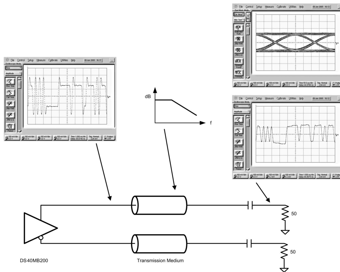
FIGURE 4. Pre-Emphasis Waveforms Before and after a Lossy Transmission Line
