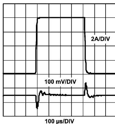
FIGURE 9. V_{IN} = 8V , V_{OUT} = 3.3V I_{LOAD} = 2A\text{ to }10A CH1: V_{OUT} , CH2: I_{LOAD}
