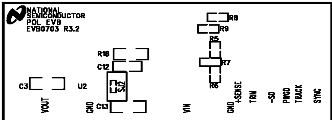
FIGURE 14. Bottom Silkscreen
