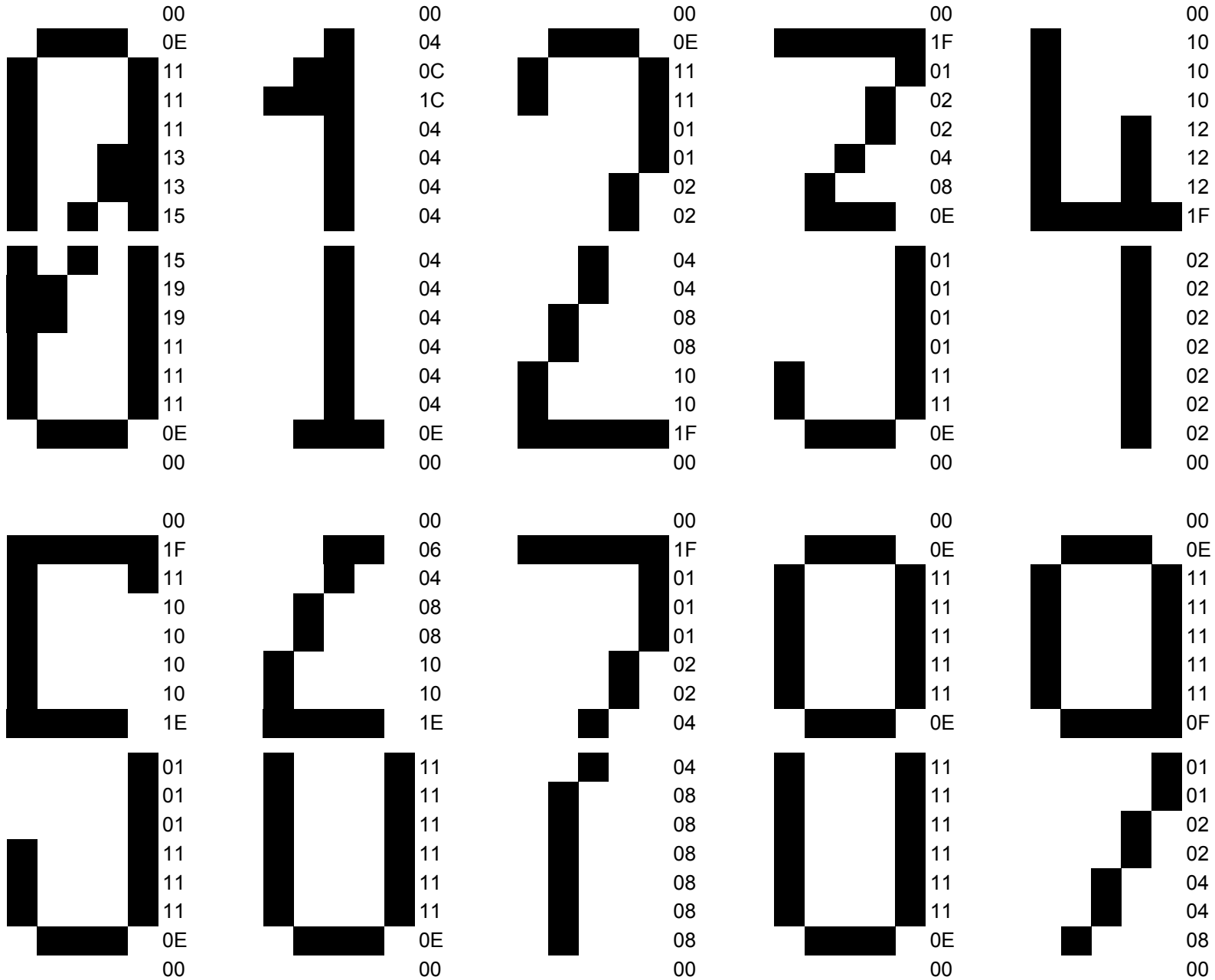
The sets of two custom characters that are needed to define the 10 double height digits. Only 8 programmable characters available, so reprogram on the fly to display up to four unique digits simultaneously.
