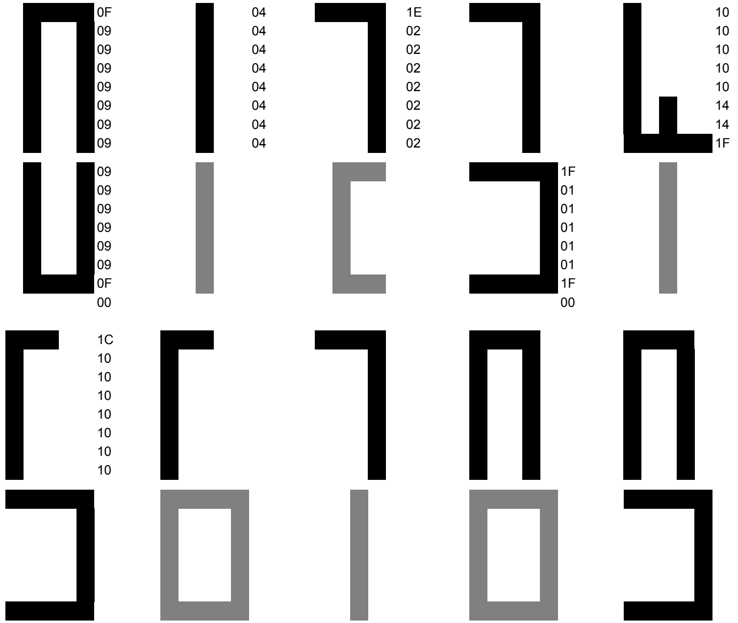
Double height digits implemented using seven custom 5x8 characters, and three existing 5x7 characters
