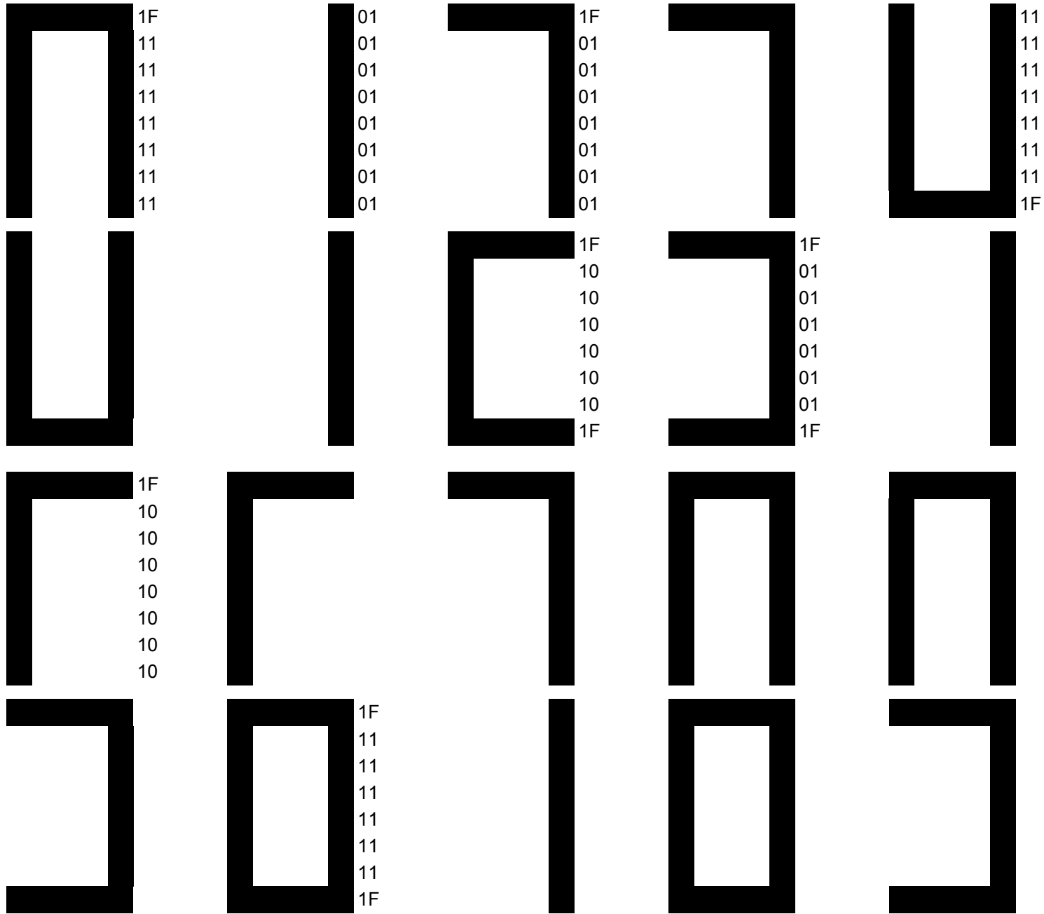
Double height digits implemented using eight custom 5x8 characters
