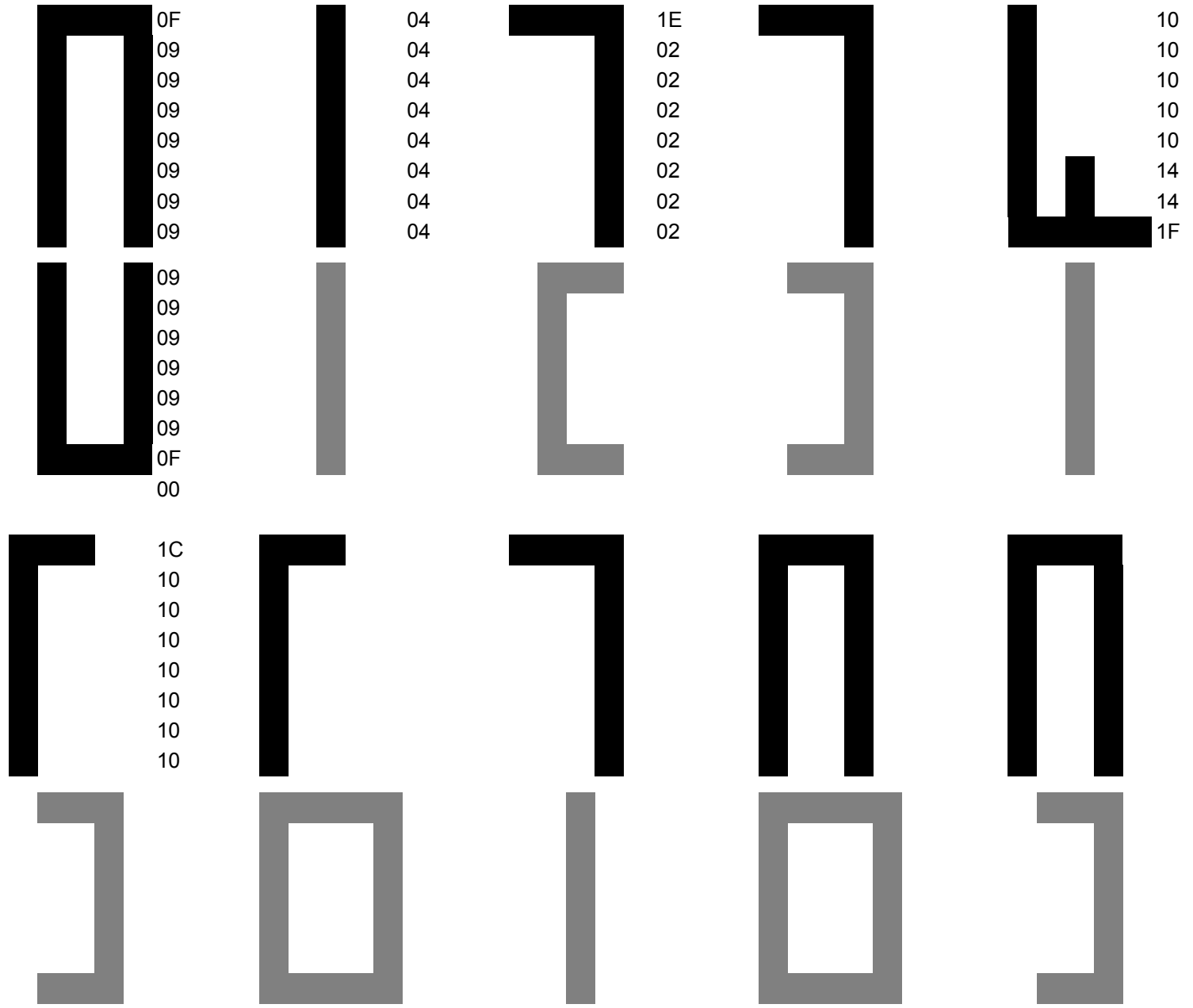
Double height digits implemented using six custom 5x8 characters, and four existing 5x7 characters
