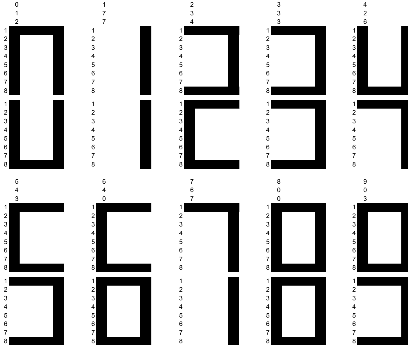
Double height digits implemented using seven custom 5x8 characters
