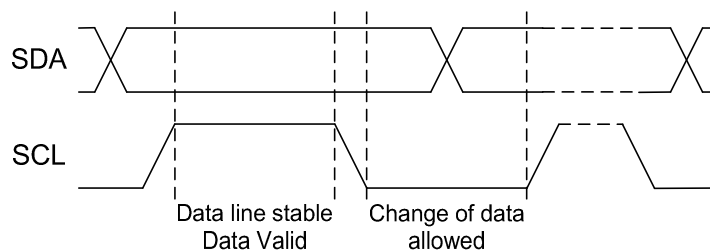
Figure 3 Bit Transfer
