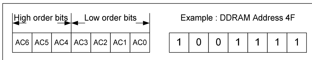
Figure 8 DDRAM Address
