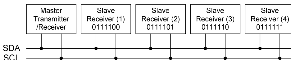
Figure 5 System Configuration
