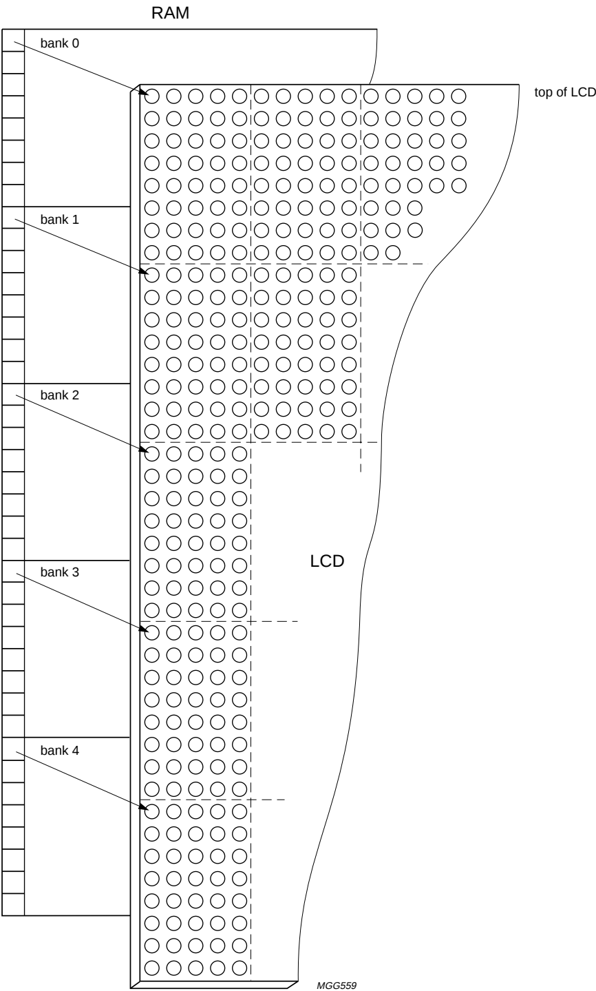
Fig.2 DDRAM to display mapping.
