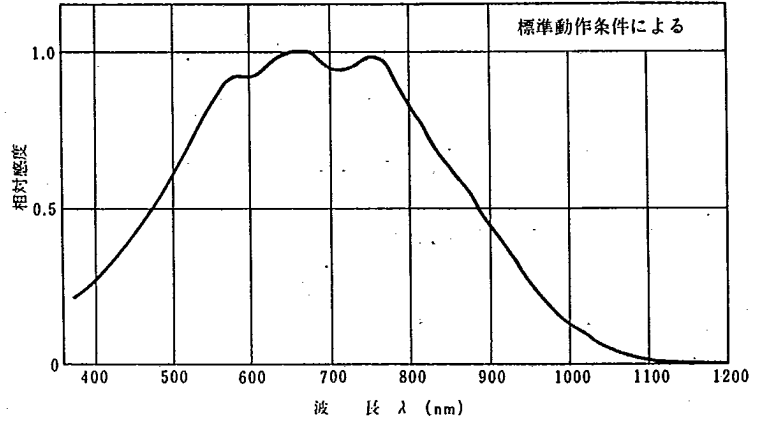
分光感度特性 / Spectral Response
